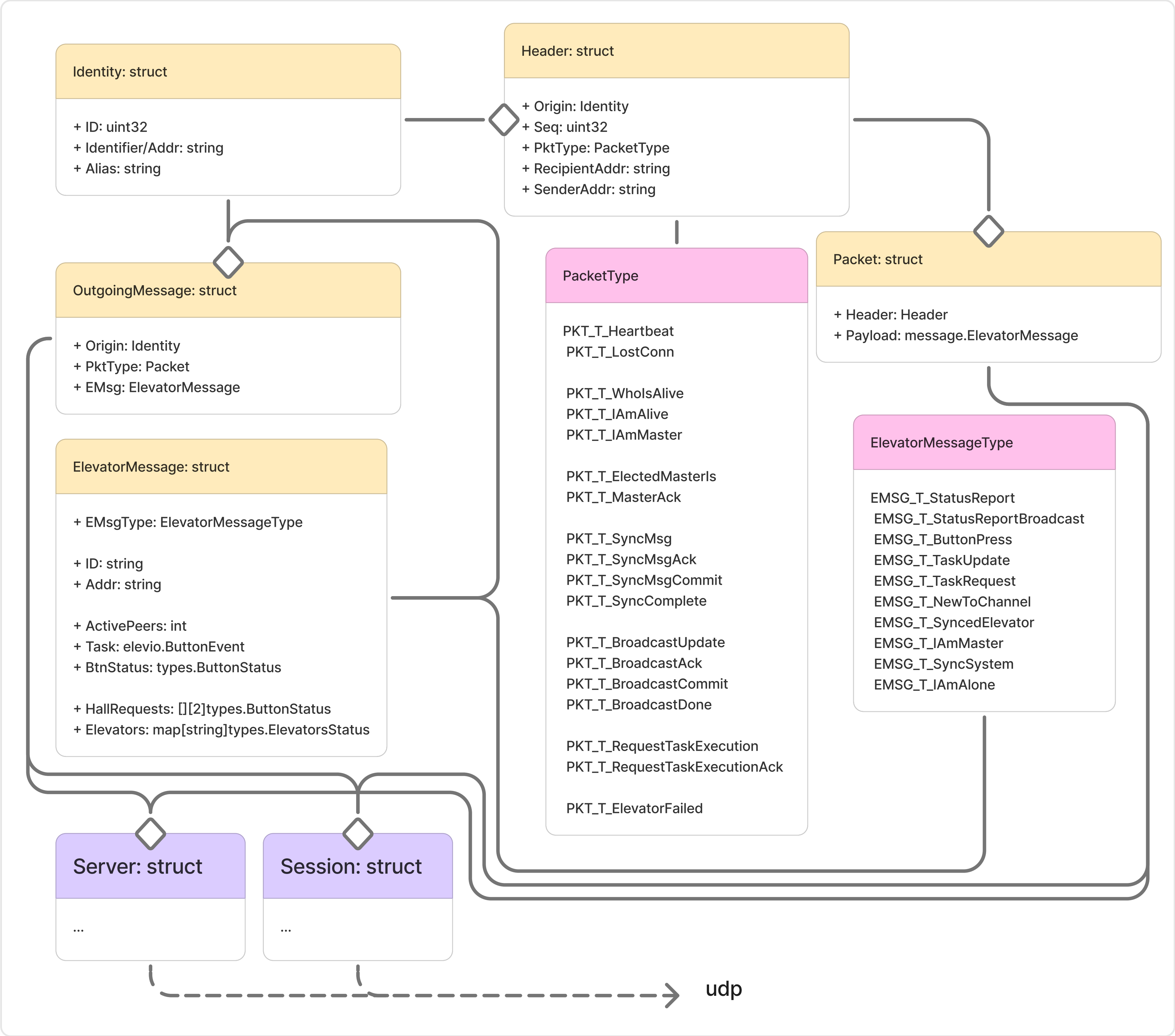
Packet - class diagram
